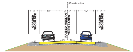
E. AVENUE 2 LANE ROADWAY
