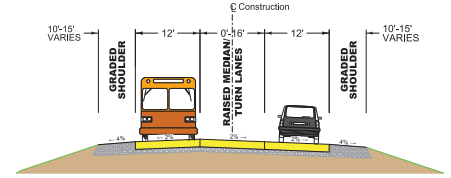
COVINGTON ROAD 2 LANE ROADWAY
