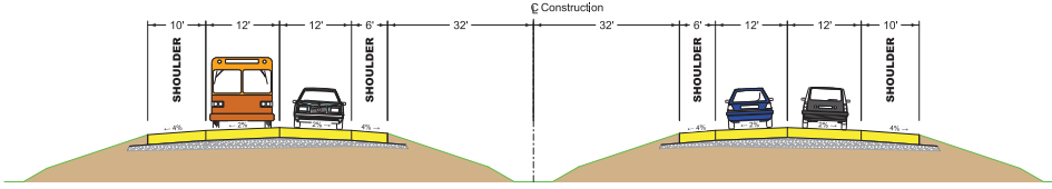
IA 100 - RURAL - TYPICAL SECTION 4-LANE DIVIDED ROADWAY
