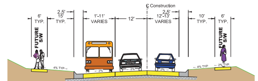
USHERS FERRY ROAD 2 LANE ROADWAY
