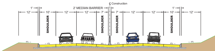
IA 100 - URBAN - TYPICAL SECTION 4-LANE UNDIVIDED ROADWAY
