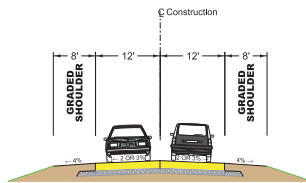
ACCESS ROAD 2 LANE ROADWAY
