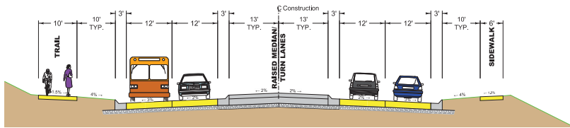
EDGEWOOD ROAD 4 LANE DIVIDED ROADWAY
