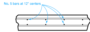
DETAIL 'A' PARTIAL LONGITUDINAL SECTION
