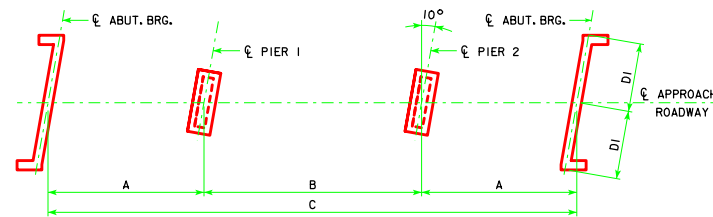
10° SKEW (L.A.)
