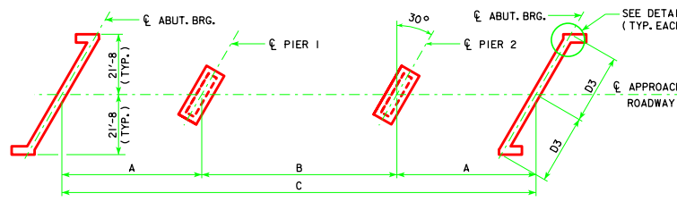
30° SKEW (L.A.)
