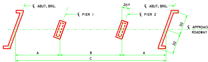
20° SKEW (L.A.)
