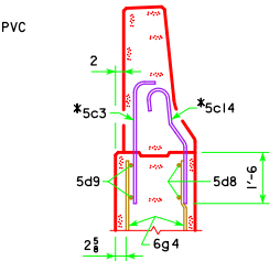
PART SECTION C-C
