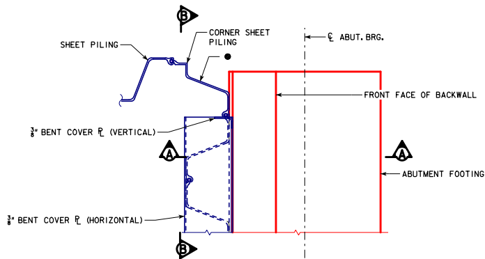
PARTIAL PLAN VIEW AT END OF ABUTMENT
