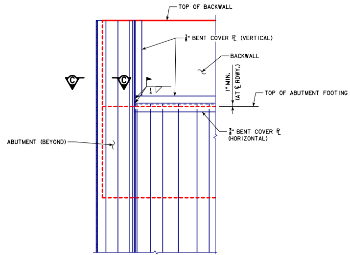
VIEW B-B
