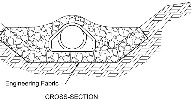
CROSS-SECTION
