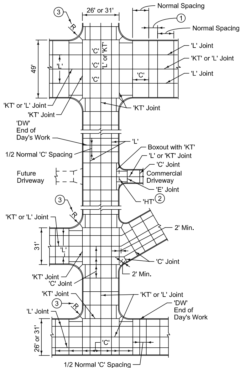
PLAN VIEW
