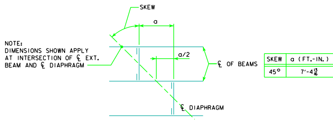
45° SKEWED FRAMING PLAN (R.A. SHOWN, L.A. SIMILAR)
