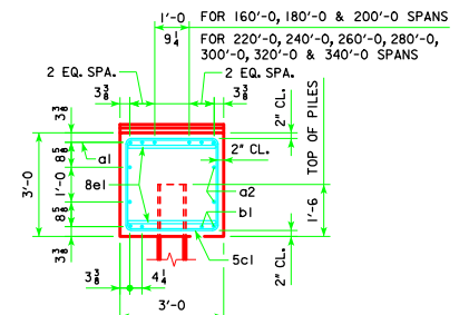
VIEW A-A FOR 14, 16 & 18 PILE BENTS
