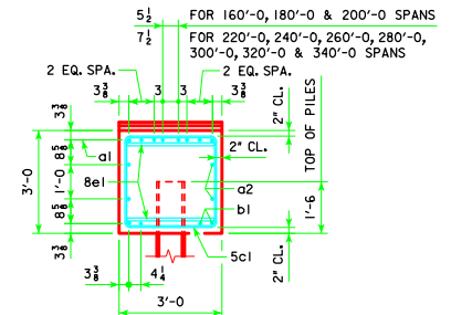
VIEW A-A FOR 10 & 12 PILE BENTS
