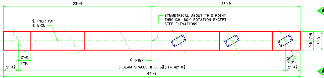
TYPICAL PLAN
