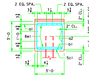
VIEW A-A FOR 9, 10, 11, 12, 13, 14 & 15 PILE BENTS
