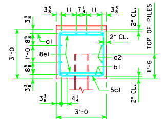
VIEW A-A FOR 16 PILE BENT
