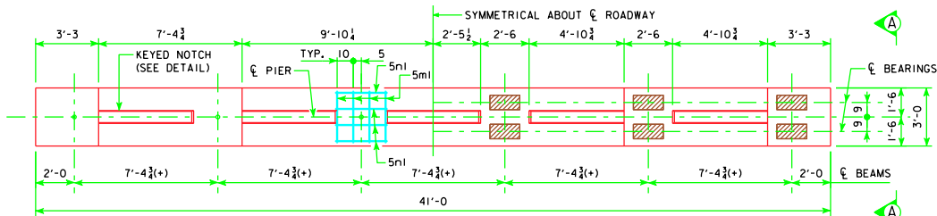
TYPICAL PLAN
