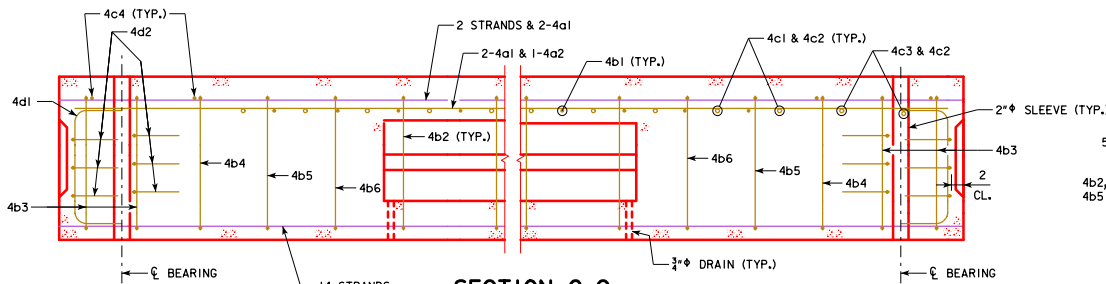
SECTION C-C (KEYWAY NOT SHOWN FOR CLARITY)
