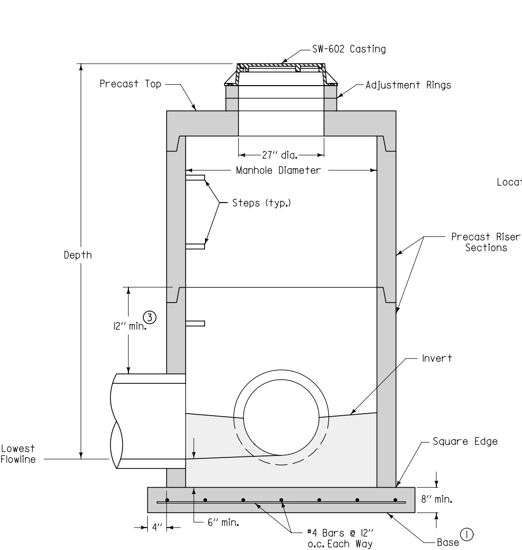
TYPICAL SECTION
