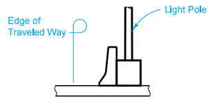
TYPE 5 Concrete Barrier Rail or Bridge Rail
