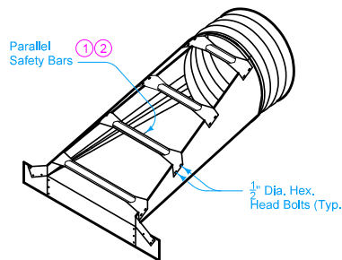
PERSPECTIVE VIEW OF APRON
