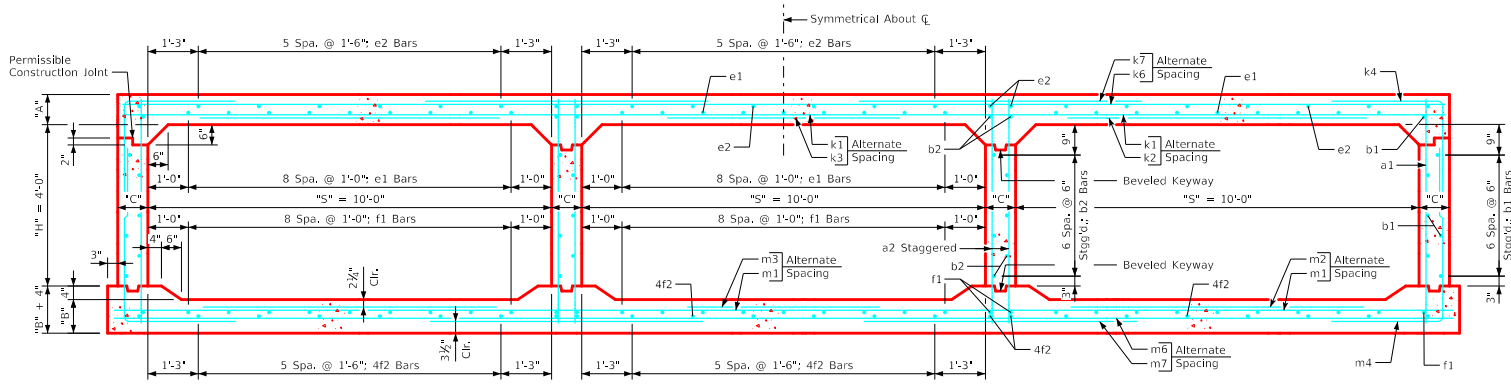
Triple 10' x 4' Barrel Section
