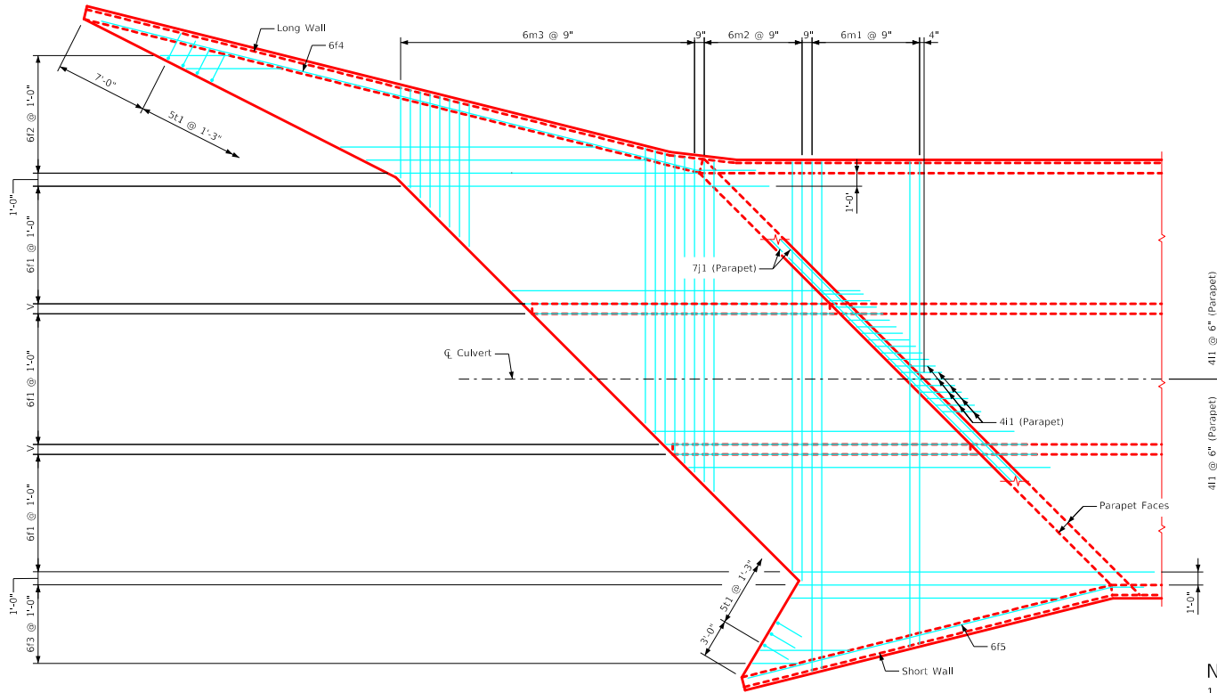
Plan View - Top of Apron Reinforcing
