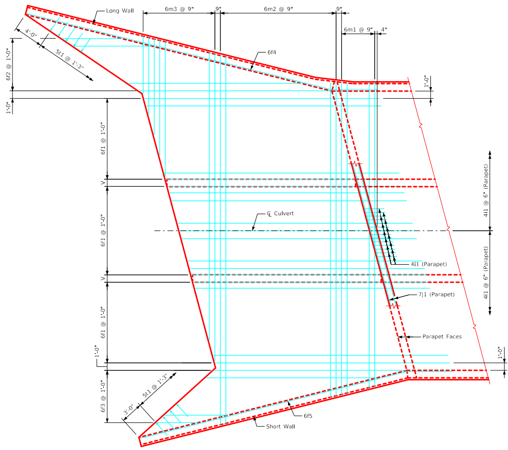
Plan View - Top of Apron Reinforcing
