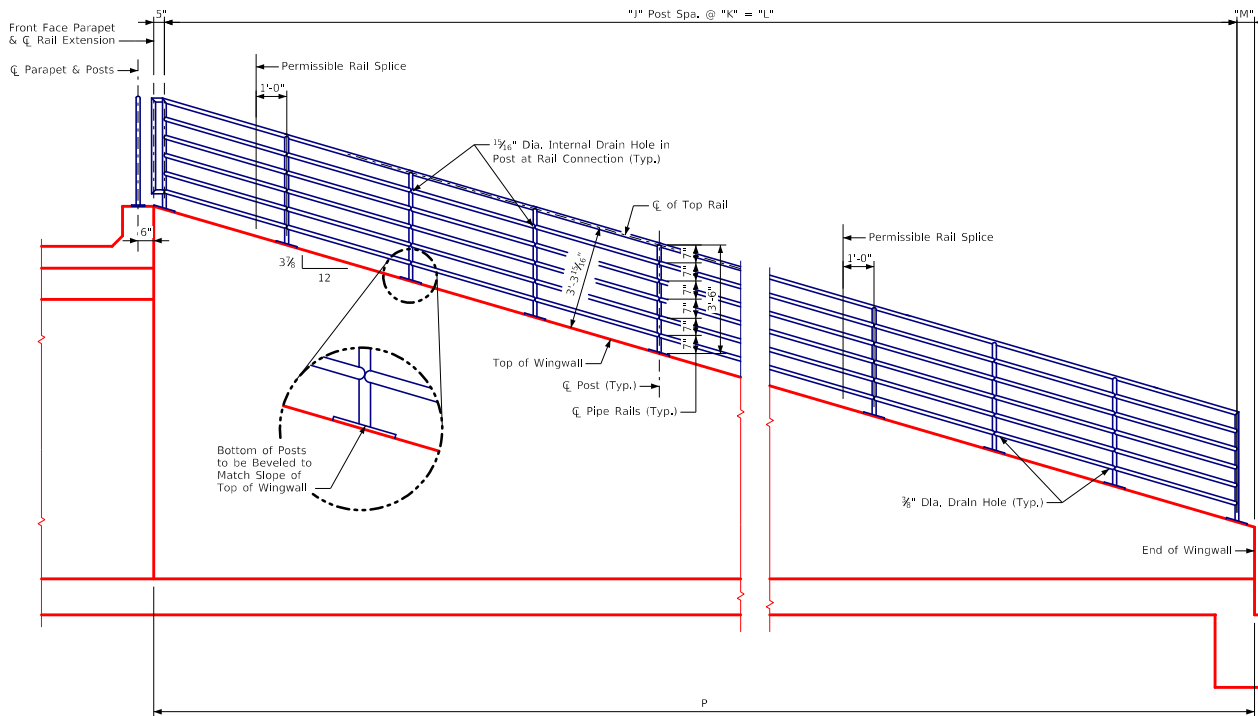
Elevation View of Wingwall
