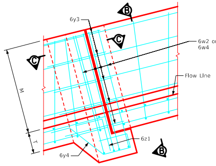
Part Elevation - Chute Bell Jt.
