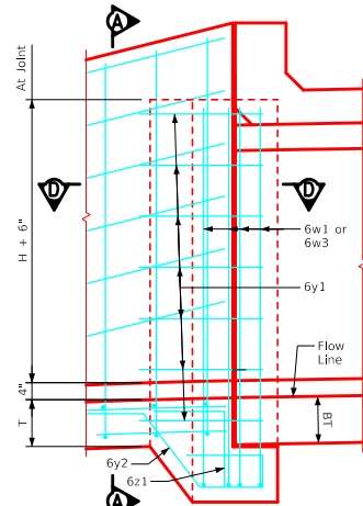
Part Elev. - Junction Bell Jt.
