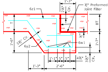
Section E-E
