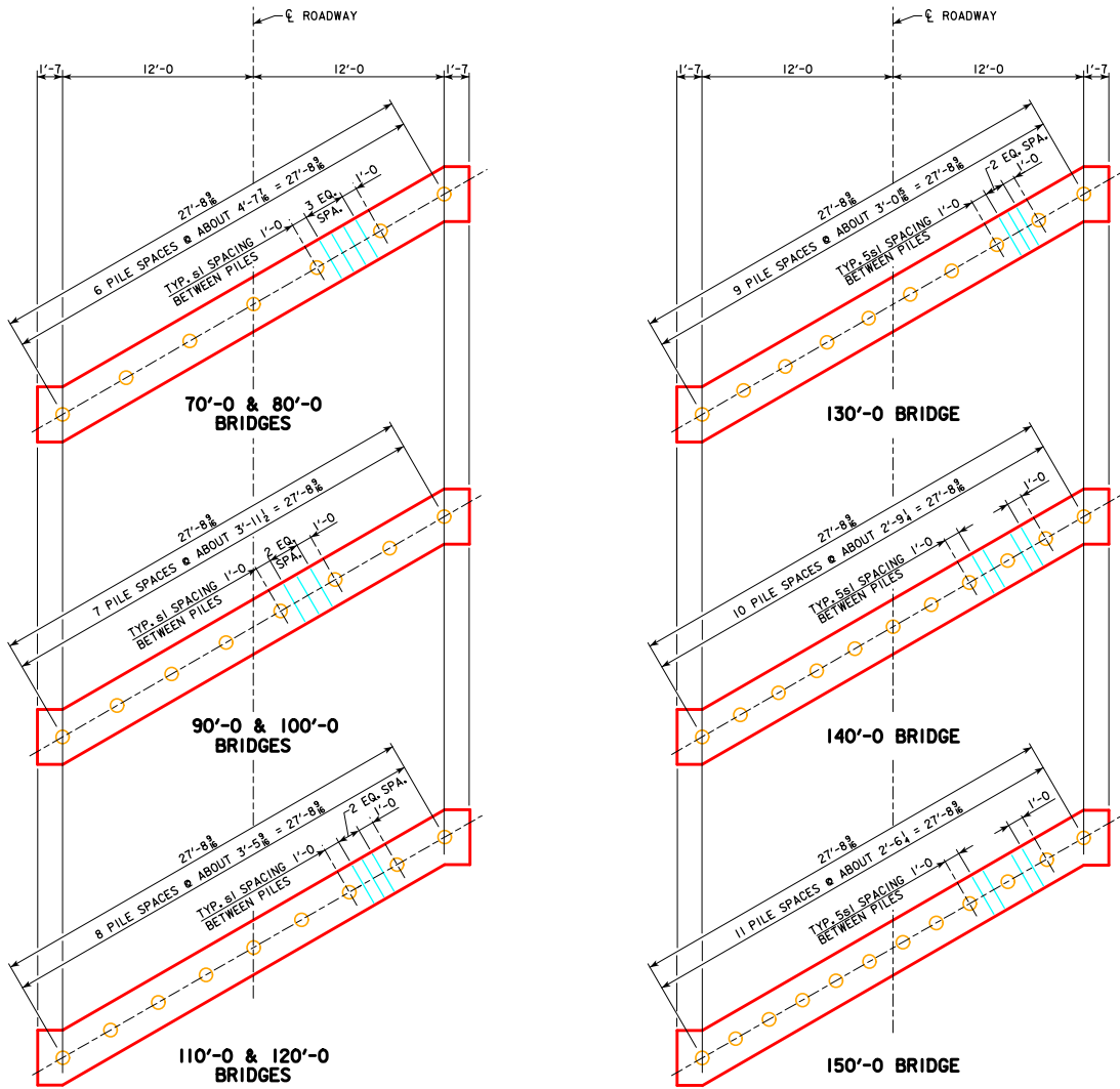
PILE PLAN - 30° SKEW WOOD PILING
