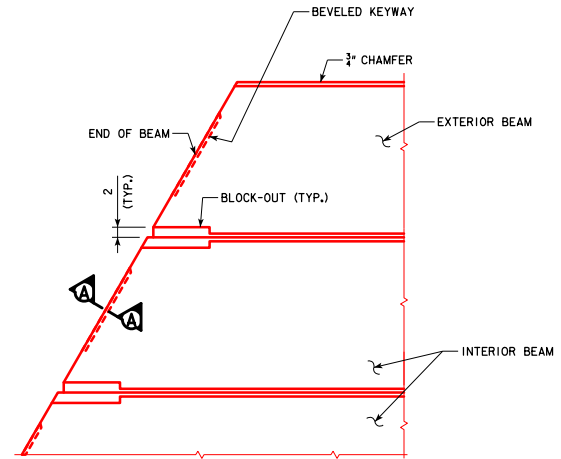
PARTIAL PLAN (30° SKEW SHOWN, 15° SKEW SIMILAR)
