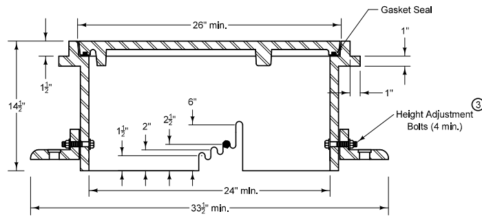
TYPICAL SECTION
