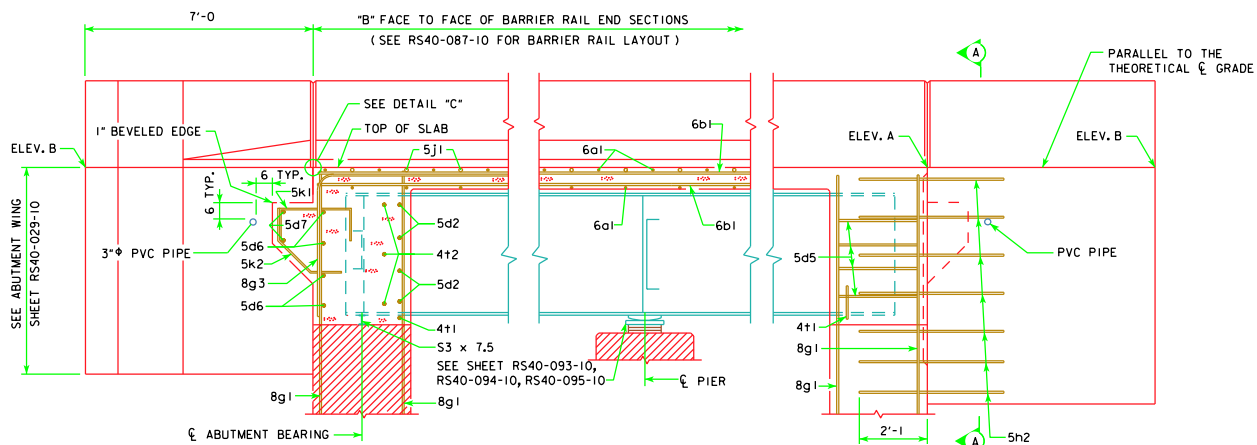
PART LONGITUDINAL SECTION NEAR GUTTER
