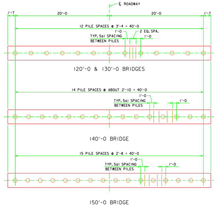
PILE PLAN - 0° SKEW WOOD PILING
