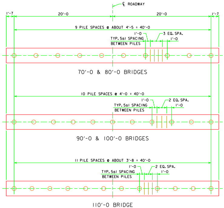
PILE PLAN - 0° SKEW WOOD PILING
