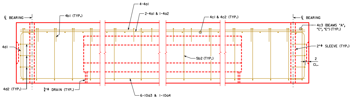
ELEVATION (KEYWAY NOT SHOWN FOR CLARITY)
