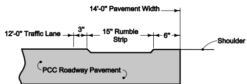
SECTION THROUGH PAVEMENT EDGE
