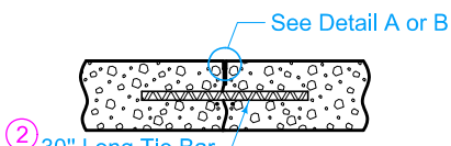
'CT' 4 TIED CONTRACTION JOINT
