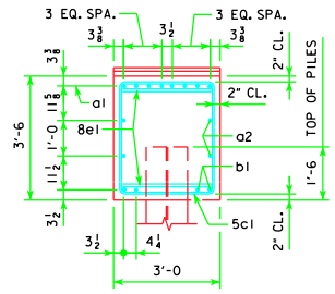
VIEW A-A FOR 7, 8, 9, 10, 11, 12 & 13 PILE BENTS
