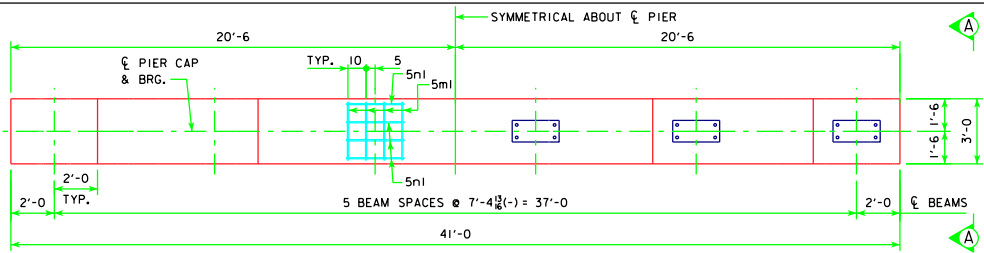
TYPICAL PLAN
