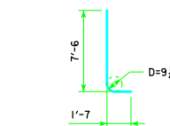
d2 NOTE: D = PIN DIAMETER. DIMENSIONS ARE OUT TO OUT.
