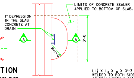
PART PLAN
