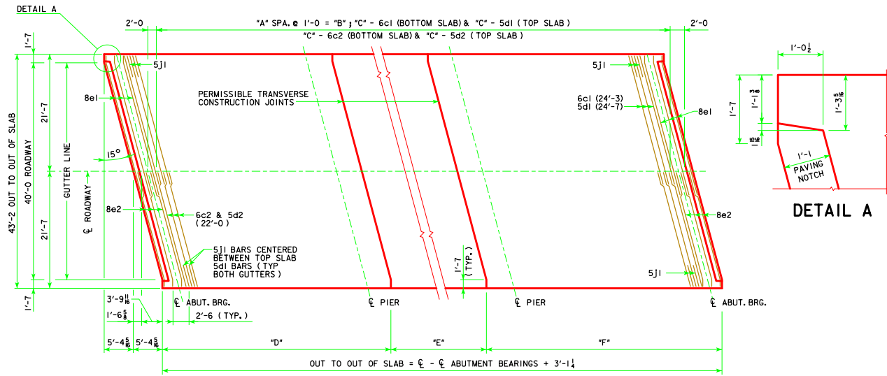
15° SKEW TRANSVERSE REINFORCING STEEL LAYOUT
