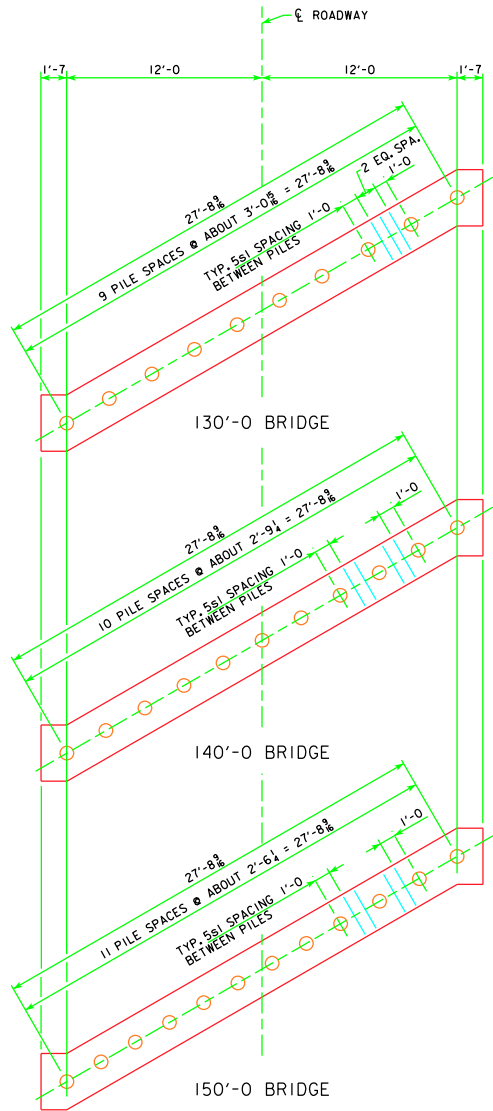
PILE PLAN - 30° SKEW WOOD PILING
