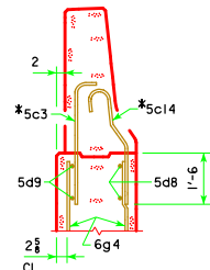
PART SECTION C-C * NOTE: SEE BARRIER RAIL SHEET FOR DETAILS. REINFORCING BARS 5c3 AND 5c14 ARE INCLUDED IN SUPERSTRUCTURE QUANTITIES.
