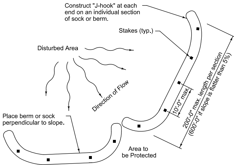
PLAN VIEW OF SLOPE (for sediment and slope control)
