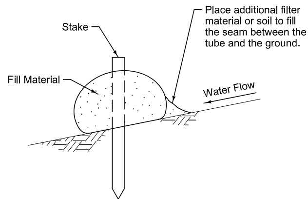
FILTER SOCK
