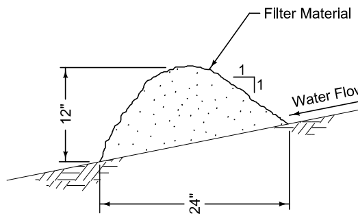
FILTER BERM
