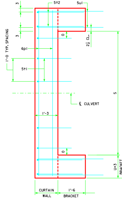
CURTAIN WALL DETAIL APRON IS NOT SHOWN
