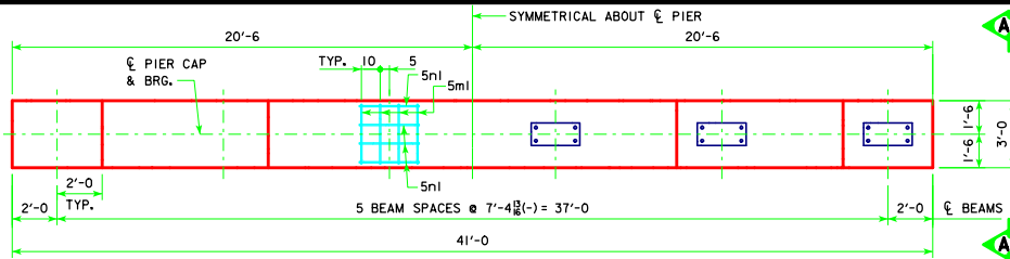
TYPICAL PLAN
