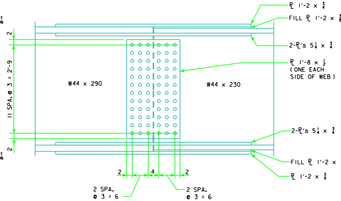
BOLTED SPLICE DETAILS
