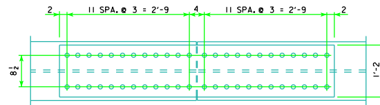
TOP AND BOTTOM FLANGE
