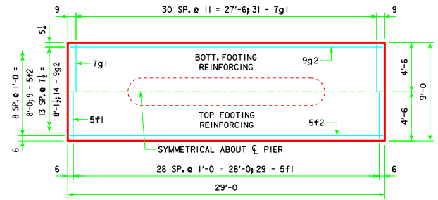
3'-6 x 9'-0 x 29'-0
