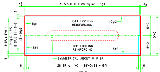
3'-6 x 10'-0 x 29'-0
