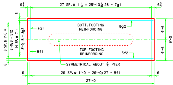
3'-6 x 9'-0 x 27'-0
