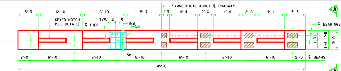
TYPICAL PLAN
