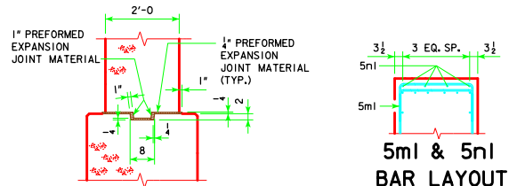
KEYED NOTCH DETAIL
