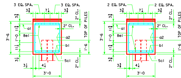
VIEW A-A FOR 7, 8, 9 & 10 PILE BENTS
