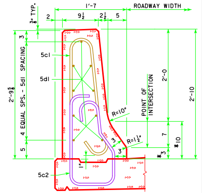
PART SECTION B-B
