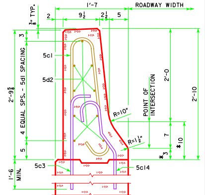
PART SECTION A-A
