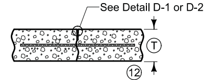
'L' CONTRACTION JOINT
