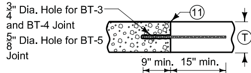
'BT' ABUTTING PAVEMENT JOINT - RIGID TIE (Drilled)
