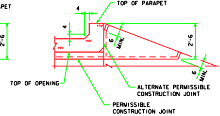
TOP OF WINGWALL DETAILS
