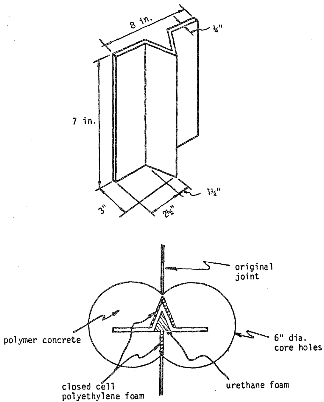
Figure 3 Vee Device
