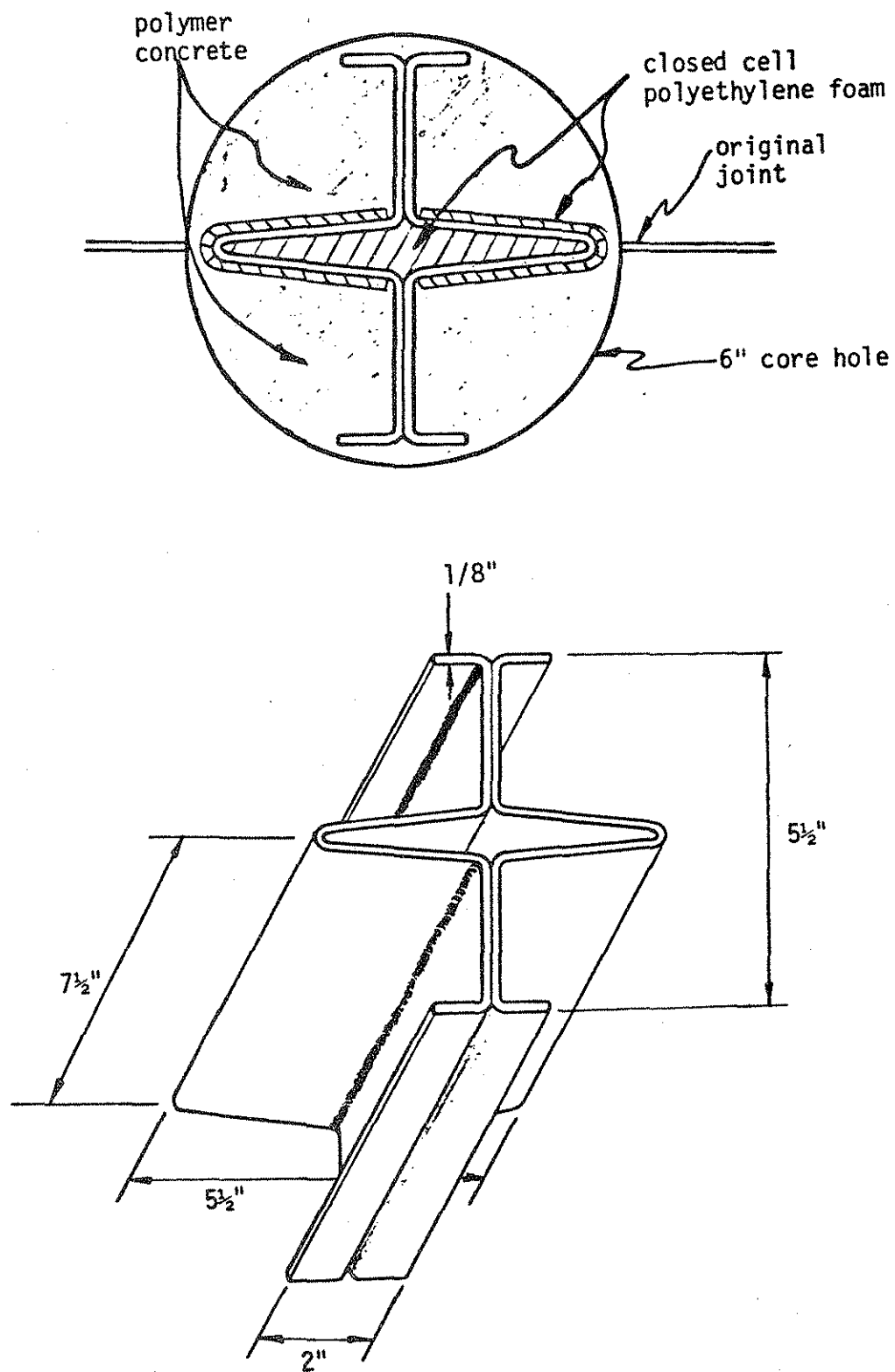
Figure 4 Double Vee Device
