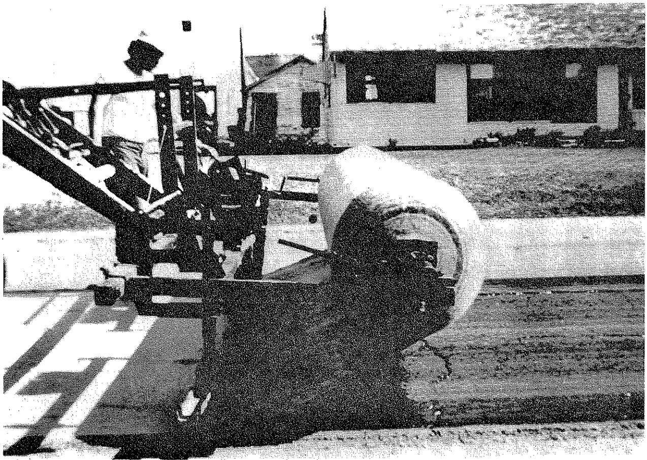
Figure 6 - Placing Reinforcing Fabric to Prevent Reflection Cracking
