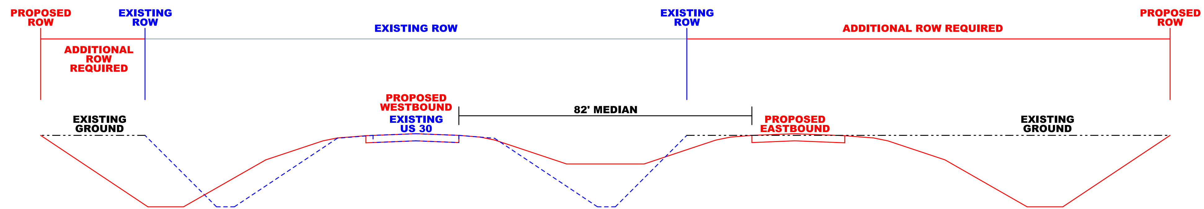
U.S. 30 BENTON COUNTY - ALTERNATIVE 3
