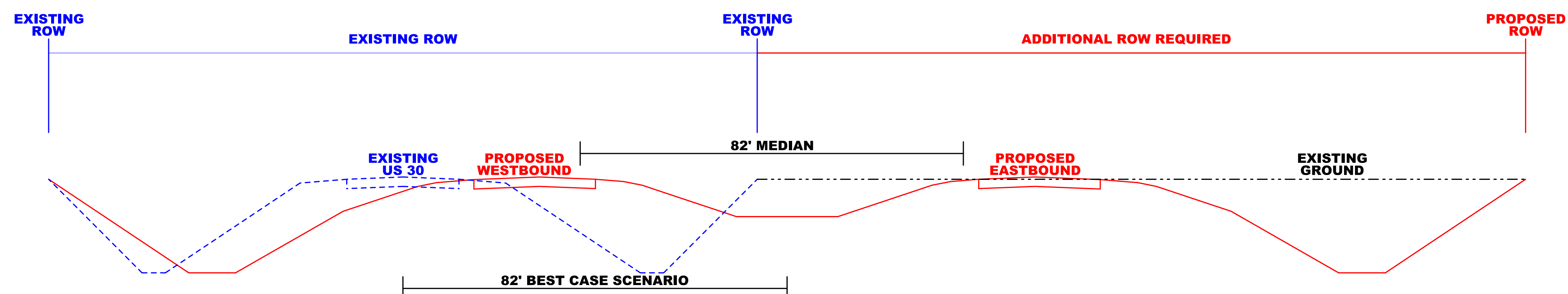
U.S. 30 BENTON COUNTY - ALTERNATIVE 1
