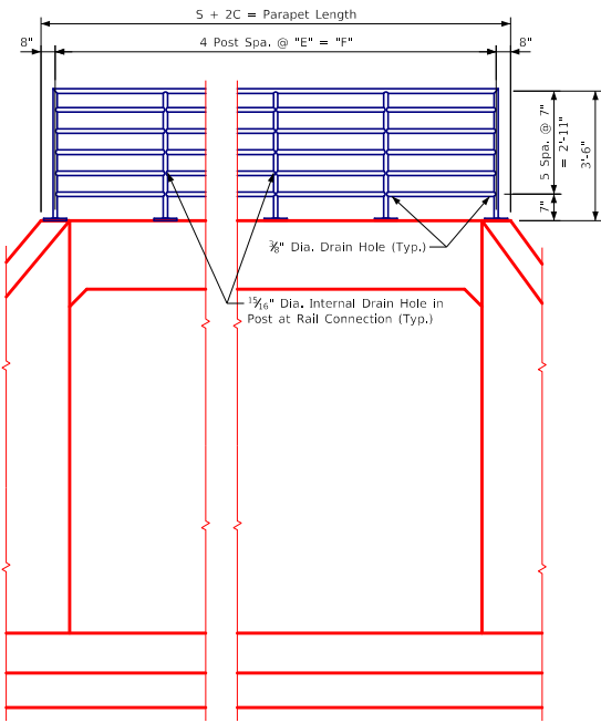
Partial End View of Parapet and Headwall
