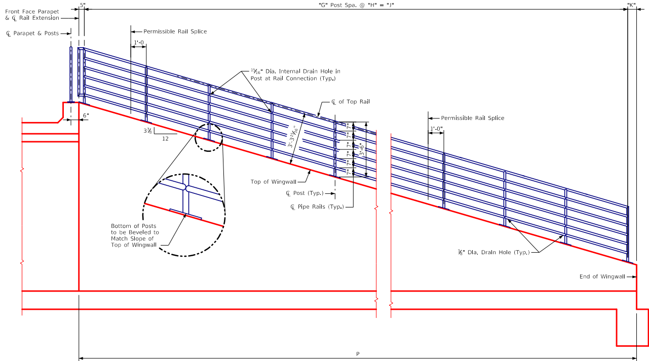
Elevation View of Wingwall
