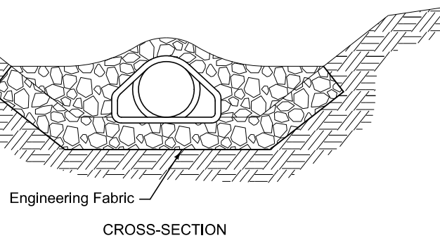
CROSS-SECTION
