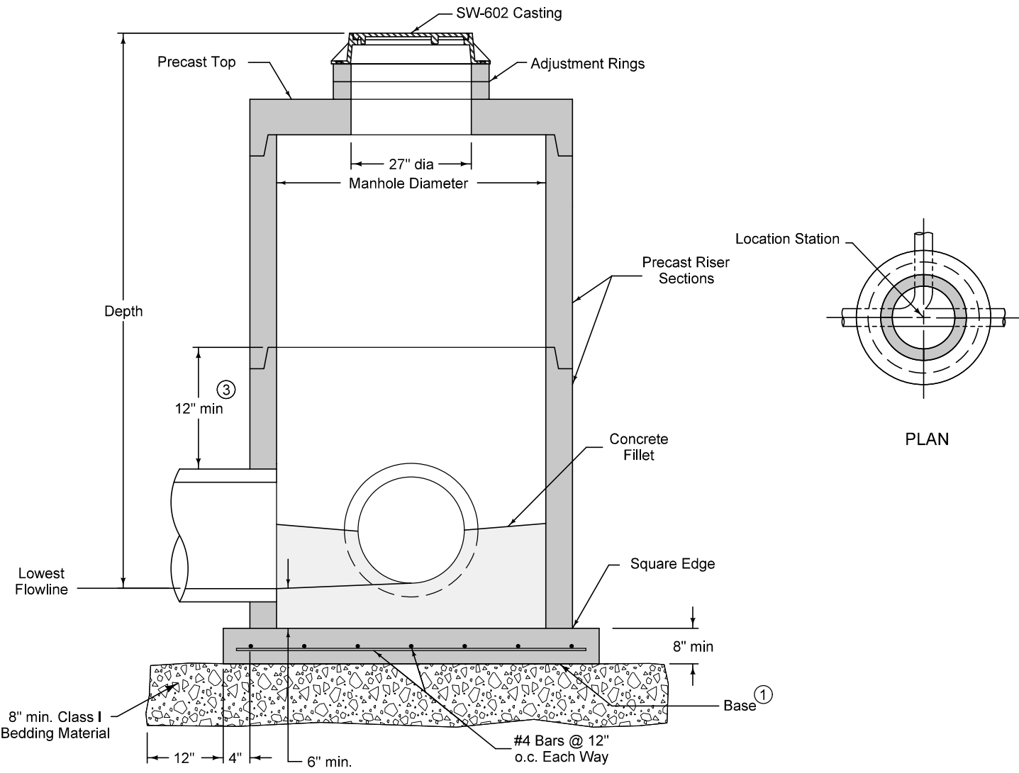
TYPICAL SECTION
