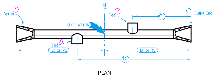
REINFORCED CONCRETE PIPE CULVERT
