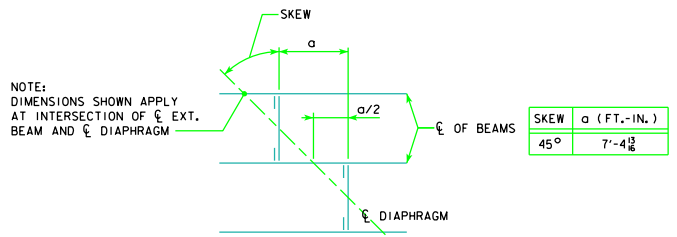
45° SKEWED FRAMING PLAN (R.A. SHOWN, L.A. SIMILAR)
