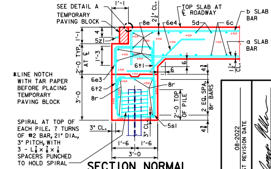
SECTION NORMAL TO ABUTMENT AT C (BRIDGE LENGTHS 120'-0 - 150'-0')
