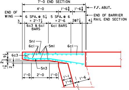
PART PLAN 15° SKEW (RAILING NOT SHOWN)
