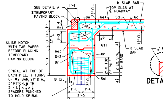
SECTION NORMAL TO ABUTMENT AT C (BRIDGE LENGTHS 70'-110')
